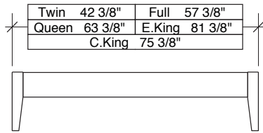
BASIC FOOTBOARD
